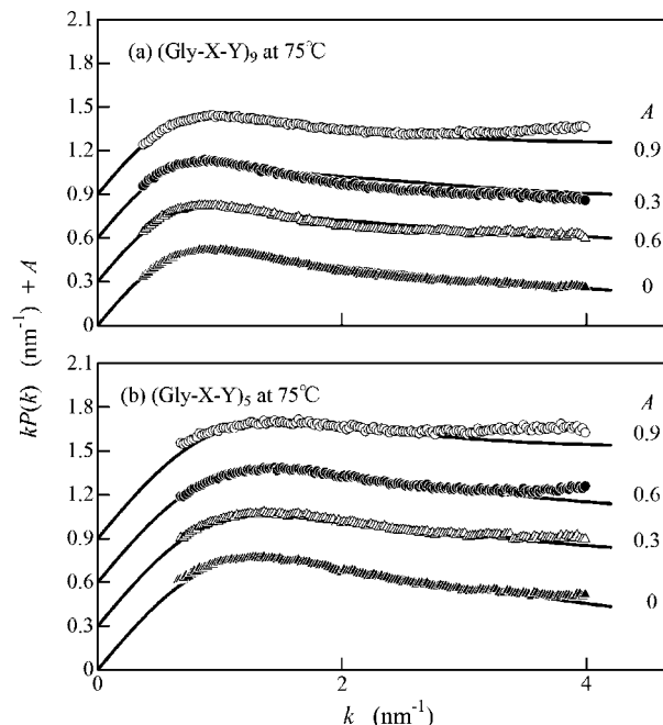
Figure 9. Holtzer plots for H-(Gly-Pro-Pro) _n -OH (open circles), H-(Gly-Hyp-Pro) _n -OH (filled circles), H-(Gly-Pro-Hyp) _n -OH (open triangles), and H-(Gly-Hyp-Hyp) _n -OH (filled triangles) in PBS at 75 °C. Curves: Nakamura–Norisuye's theoretical values for the wormlike cylinder with the common h and \lambda^{-1} of 0.33 and 2 nm, respectively, and d of 0, 0.45, 0.45, and 0.67 nm from top to bottom in each panel.
