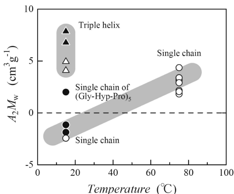
Figure 5. Temperature dependence of A_2 for collagen model peptides forming triple-helical structure (triangles) and dispersing in solution as a single molecule (circles) in pure water (filled symbols) and in PBS (open symbols).
