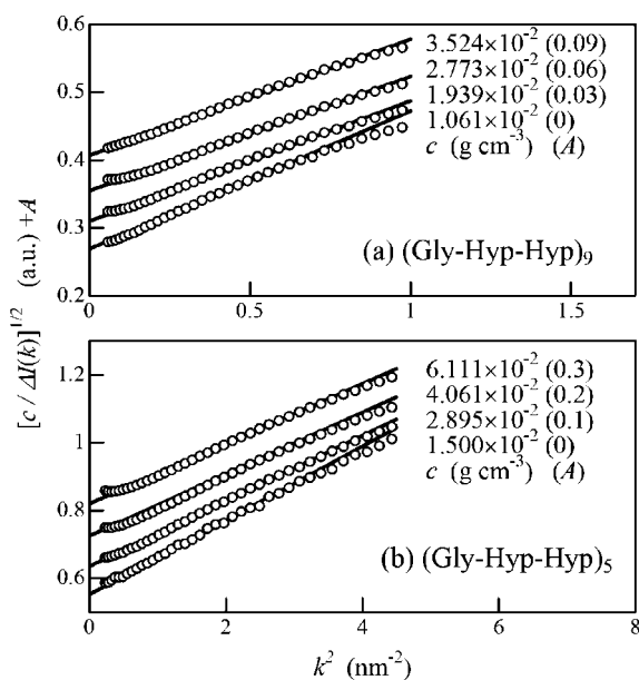
Figure 3. Berry plots for (a) H-(Gly-Hyp-Hyp) 9 -OH and (b) H-(Gly-Hyp-Hyp) 5 -OH in pure water at 15 °C. For clarity, the ordinate values of (c/\Delta I_0)^{1/2} are shifted by arbitrary constants ( A ) indicated in parentheses.
