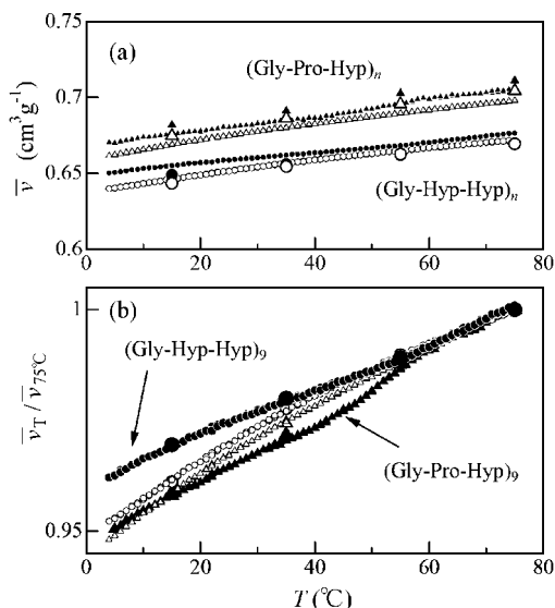
Figure 10. Temperature dependence of \bar{v} (a) and the ratio \bar{v}_T/\bar{v}_{75^\circ\text{C}} (b) for H-(Gly-Pro-Hyp) 5 -OH (open triangles), H-(Gly-Pro-Hyp) 9 -OH (filled triangles), H-(Gly-Hyp-Hyp) 5 -OH (open circles), and H-(Gly-Hyp-Hyp) 9 -OH (filled circles) in pure water. Large and small symbols are obtained from independent measurements.
