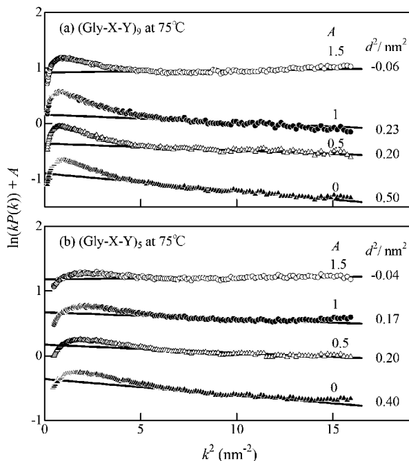
Figure 8. Cross-sectional plots for H-(Gly-Pro-Pro) _n -OH (open circles), H-(Gly-Hyp-Pro) _n -OH (filled circles), H-(Gly-Pro-Hyp) _n -OH (open triangles), and H-(Gly-Hyp-Hyp) _n -OH (filled triangles) in PBS at 75 °C. (a) H-(Gly-X-Y) _9 -OH; (b) H-(Gly-X-Y) _5 -OH. The ordinate values of \ln(kP(k)) are shifted by A .
