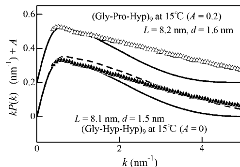
Figure 7. Holtzer plots for H-(Gly-Pro-Hyp) 9 -OH (open triangles) and H-(Gly-Hyp-Hyp) n -OH (filled triangles) in PBS at 15 °C. Solid curves, theoretical values for straight cylinders calculated from eq 5 with the indicated parameters. Dashed curve, values for the crystal structure computed by CRY SOL (ref 33) using the coordinates of the modified 1YM8 (see text). The ordinate values of kP(k) are shifted by A .
