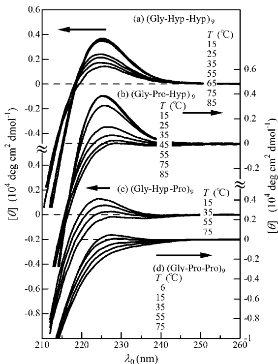
Figure 1. Circular dichroism spectra of (a) H-(Gly-Hyp-Hyp) 9 -OH, (b) H-(Gly-Pro-Hyp) 9 -OH, (c) H-(Gly-Hyp-Pro) 9 -OH, and (d) H-(Gly-Pro-Pro) 9 -OH in PBS at indicated temperatures. Peptide concentration = (1-3) \times 10^{-4} g cm -3 .
