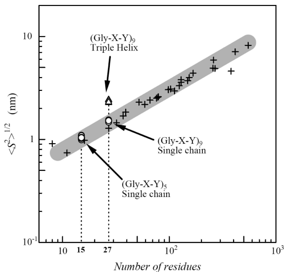
Figure 6. \langle S^2 \rangle^{1/2} for the collagen model peptides in pure water and in PBS at 15, 70, and 75 °C plotted against the number of residues. Triangles, peptides forming triple-helical structure; circles, peptides dispersing in solution as a single molecule; crosses, literature data for chemically denatured proteins (ref 34).
