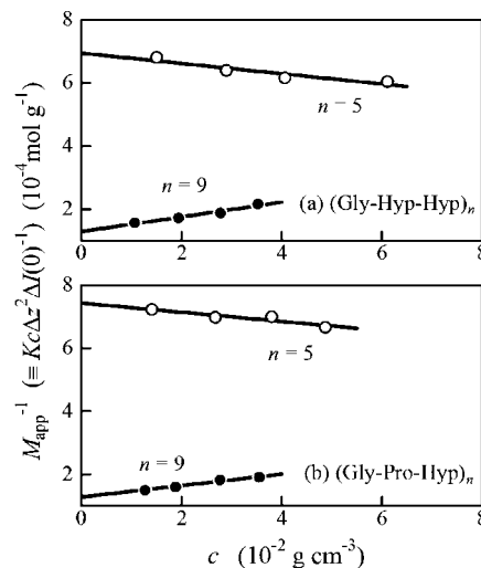
Figure 4. Concentration dependence of M_{\text{app}} for (a) H-(Gly-Hyp-Hyp) n -OH and (b) H-(Gly-Pro-Hyp) n -OH, both in pure water. Open and filled symbols indicate n = 5 and 9 , respectively.
