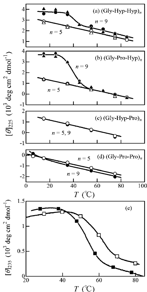
Figure 2. Temperature dependence of [\theta] for (a) H-(Gly-Hyp-Hyp) n -OH, (b) H-(Gly-Pro-Hyp) n -OH, (c) H-(Gly-Hyp-Pro) n -OH, and (d) H-(Gly-Pro-Pro) n -OH in pure water (triangles) and in PBS (circles) at the wavelength of 225 nm. Peptide concentration = (1-3) \times 10^{-4} g cm -3 . Open and filled symbols indicate n = 5 and 9 , respectively. (e) High peptide concentration ( 3.9 \times 10^{-3} g cm -3 ) data for H-(Gly-Hyp-Hyp) 9 -OH (open squares) and H-(Gly-Pro-Hyp) 9 -OH (filled squares) in water.
